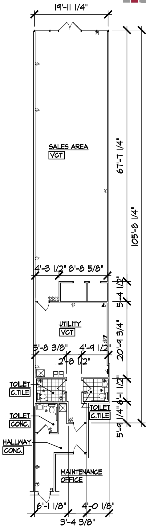
FLOOR PLAN SCALE: 1/16" = 1'-0"
