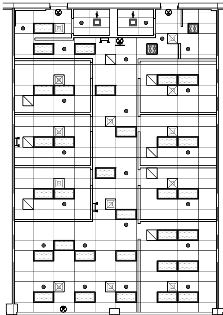
CEILING PLAN SCALE: 3/32" = 1'-0"
