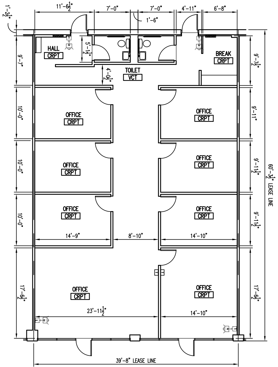
FLOOR PLAN SCALE: 3/32" = 1'-0"
